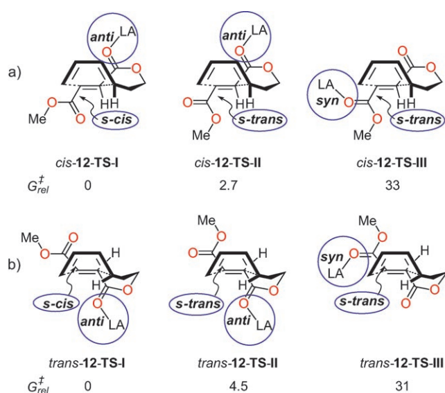
Figure 3. Relative free energies ( \text{kJ mol}^{-1} ) for selected a) cis -TSs and b) trans -TSs for fumarate 12 (LA = 1b ·H + ).
